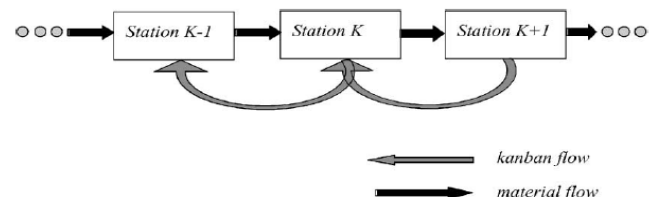
Fig. 1. Mechanism of the material and message flow in a Pull-type manufacturing system [3] Just in time (JIT) manufacturing systems produce according to production schedule, which is generated by ERP (enterprise resource planning) systems based on
