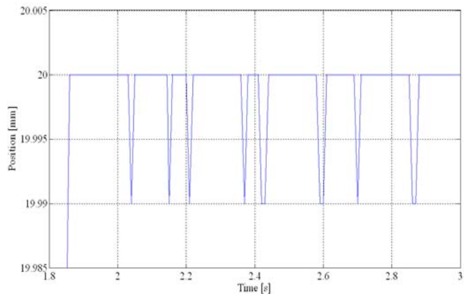
Figure 6. Position as a function of time (enlarged)
