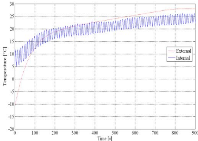
Figure 8. Temperature as a function of time with spline interpolation for internal temperature
