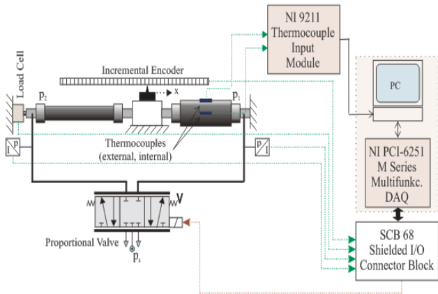
Figure 2. Block diagram of positioning system with proportional valve
