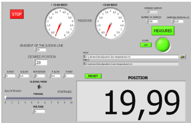
Figure 3 Front panel of LabVIEW program for positioning
