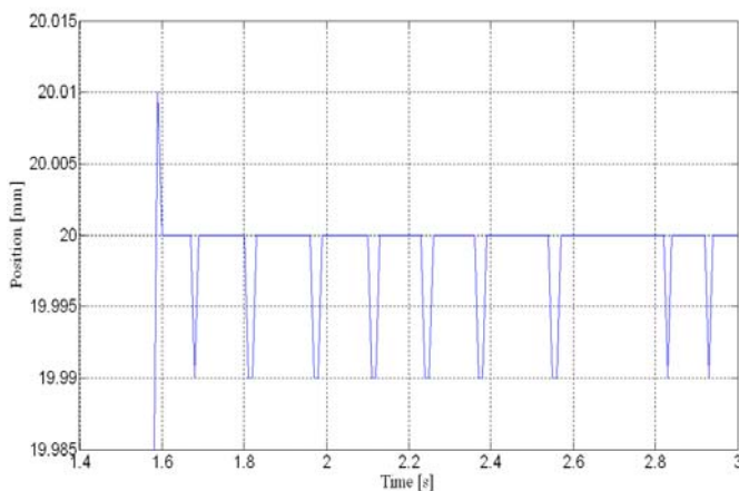
Figure 10. Position as a function of time (enlarged) after work cycle
