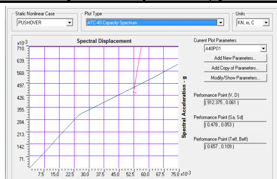
Figure 4. Pushover curve
