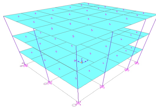
Figure 3. 3-D View
