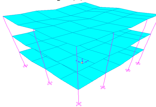
Figure 2. Deformed shape (DEAD)
