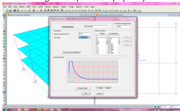
Figure 3. Response spectrum
