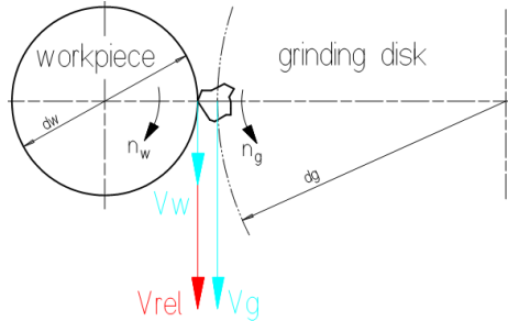
Figure 9 – Relative velocity
