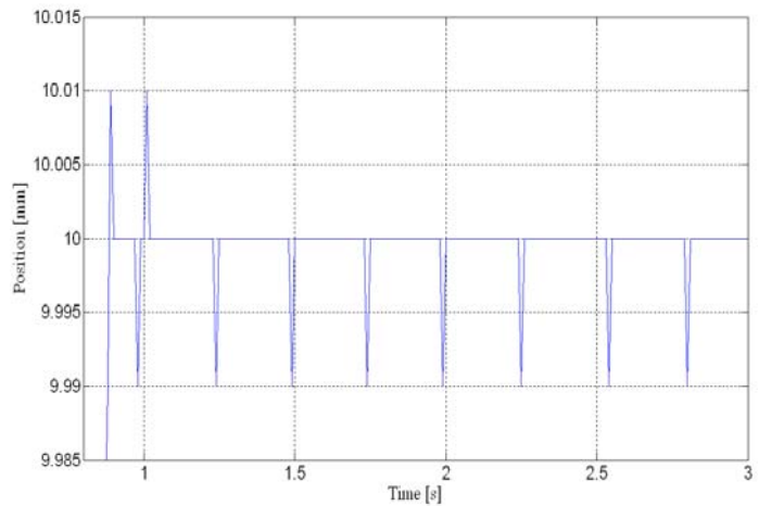
Figure 16 Position as a function of time (enlarged) after work cycle
