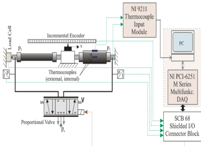
Figure 2 Block diagram of positioning system with proportional valve
