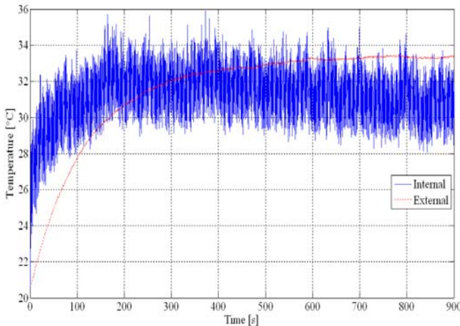
Figure 7 Temperature as a function of time
