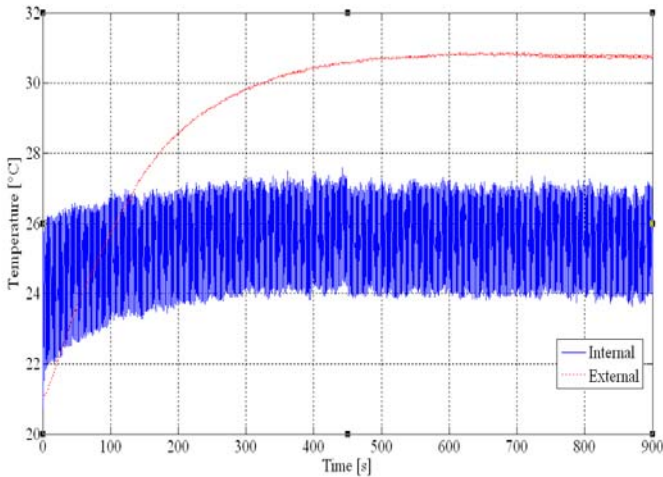
Figure 13 Temperature as a function of time
