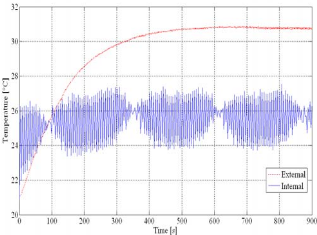
Figure 14 Temperature as a function of time with spline interpolation for internal temperature
