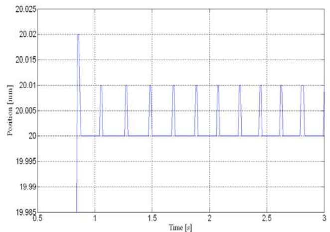
Figure 10 Position as a function of time (enlarged) after work cycle
