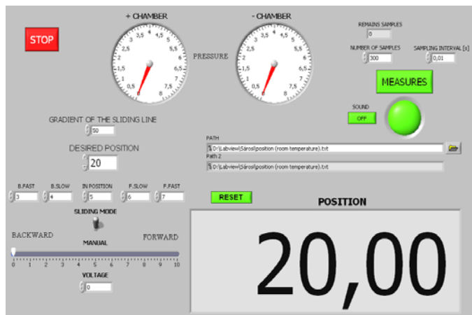
Figure 3 Front panel of LabVIEW program for positioning
