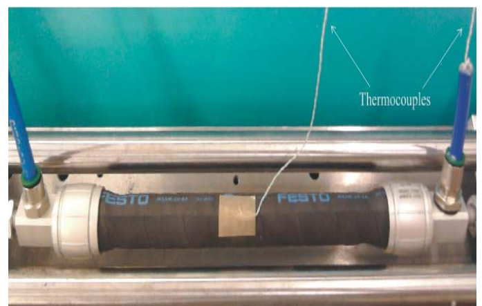
Figure 1 Muscle with two thermocouples
