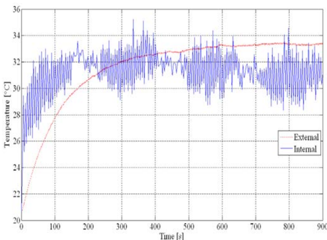
Figure 8 Temperature as a function of time with spline interpolation for internal temperature
