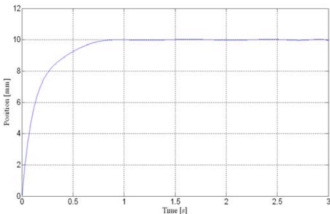
Figure 15 Position as a function of time after work cycle
