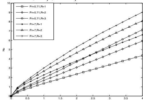
Figure 10: Nusselt Number
