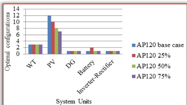
Figure 5: Variation of the rated power of SECS for the AP120 module
