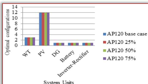
Figure 7: Variation of the rated power of storage for the AP120 module
