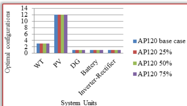
Figure 6: Variation of the rated power of DG for the AP120 module
