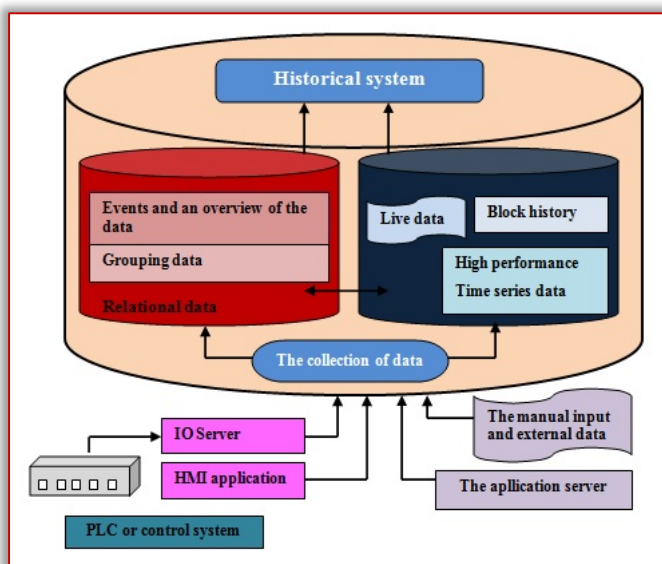
Figure 5: Architecture of the database with historical data
