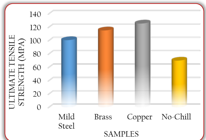
Figure 5: Chart of ultimate tensile strength of samples with different chill materials
