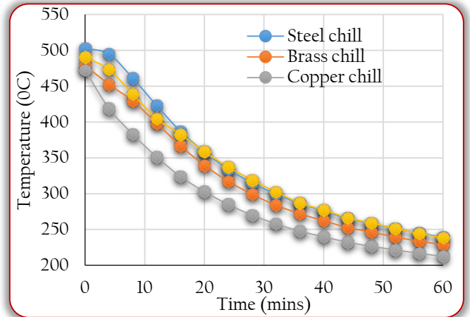
Figure 4: Cooling curves of aluminium alloy during solidification
