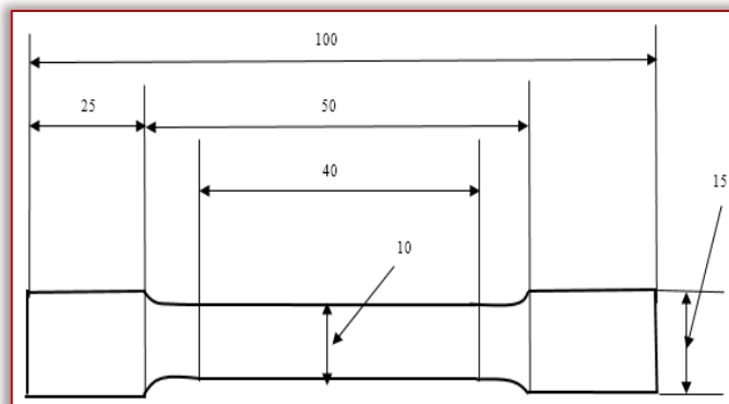
Figure 3: Dimension of the tensile test sample (mm)
