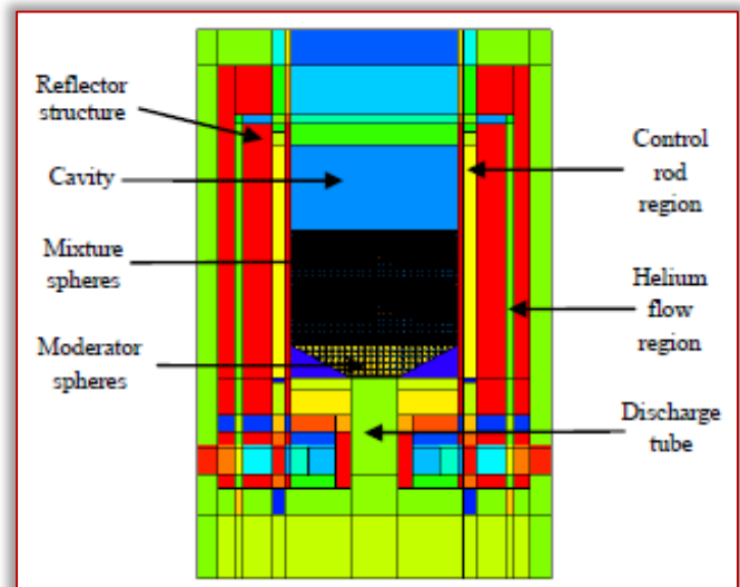
Figure 2. MCNP6 Model of HTR–10 (Vertical Cross Section)
