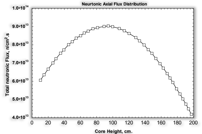
Figure 12. Axial total flux distribution for HTR-10 versus core height
