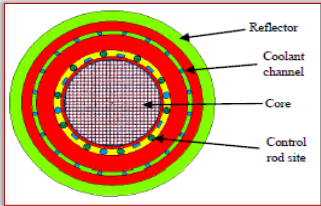
Figure 3. MCNP6 Model of HTR-10 (Horizontal Cross Section)
