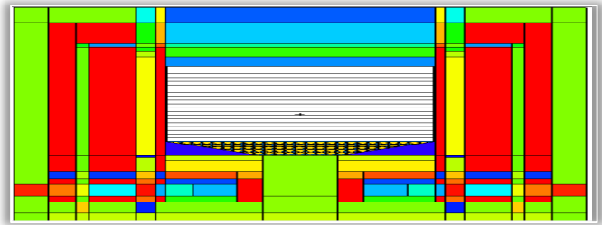
Figure 10. Axial zones for HTR-reactor
