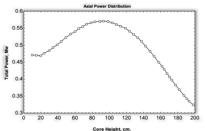
Figure 13. Axial total power distribution for HTR-10 versus core height
