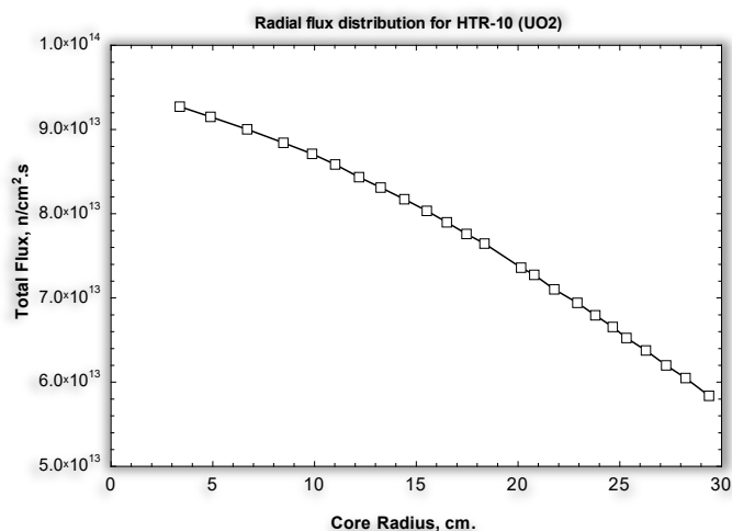
Figure 8. Radial total flux distribution for HTR-10 versus core radius
