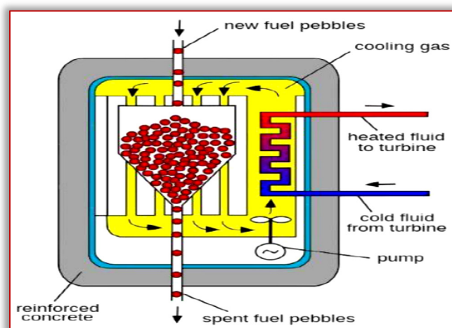
Figure 1: Schematic of the pebble bed reactor [4].
