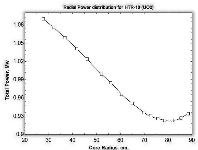
Figure 9. Radial total power distribution for HTR-10 versus core radius
