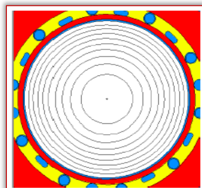
Figure 5. Radial zones for HTR-reactor
