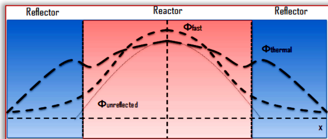
Figure 7. Effect of reflection in the thermal reactor
