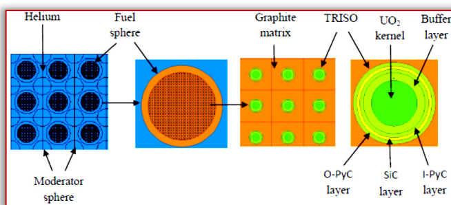
Figure 4. Pebble-bed and moderator ball in a BCC lattice and TRISO in the reactor core model.
